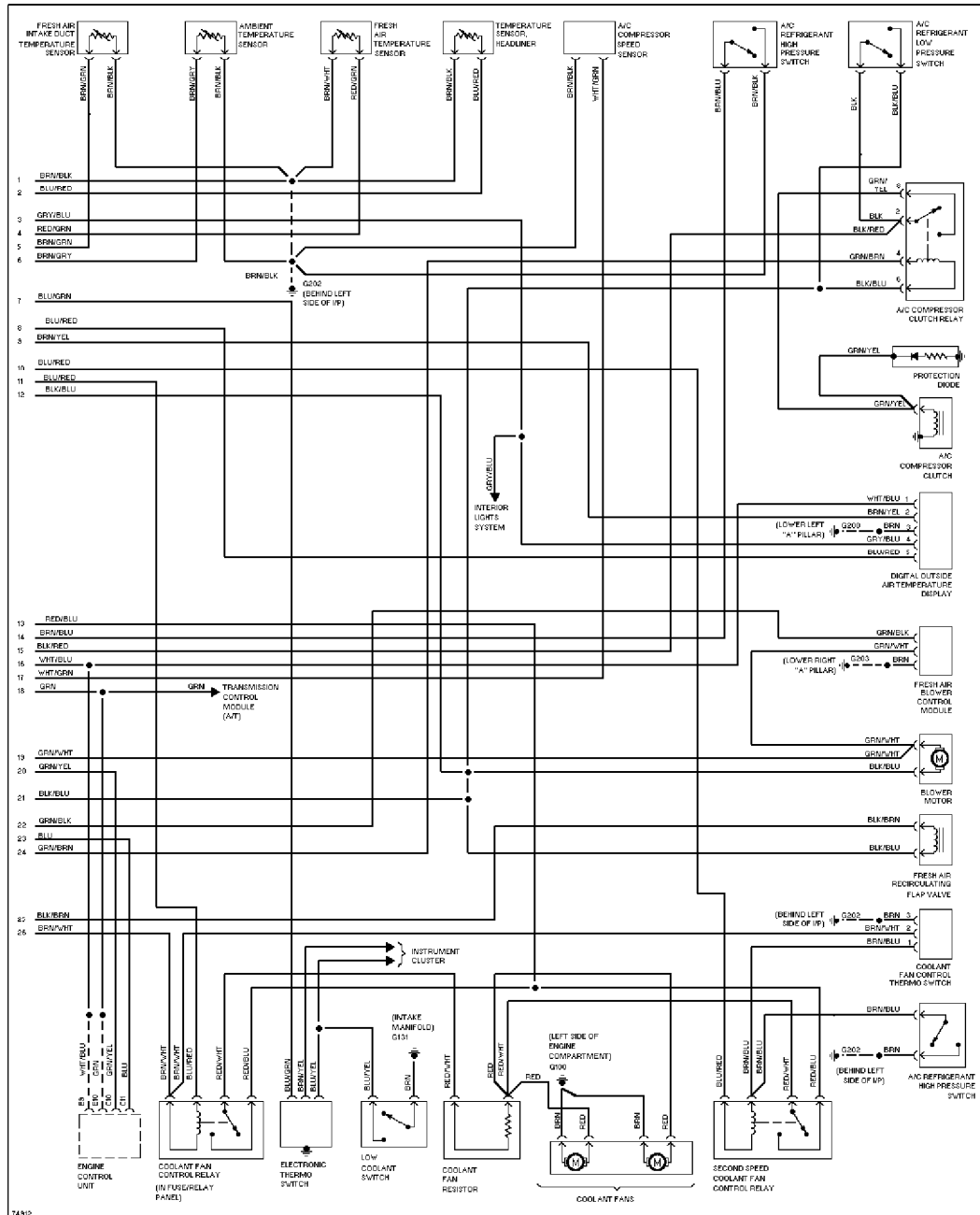
Fig. 7: Automatic A/C-Heater System Wiring Diagram (1995 (Early Production) - 2 Of 2)
