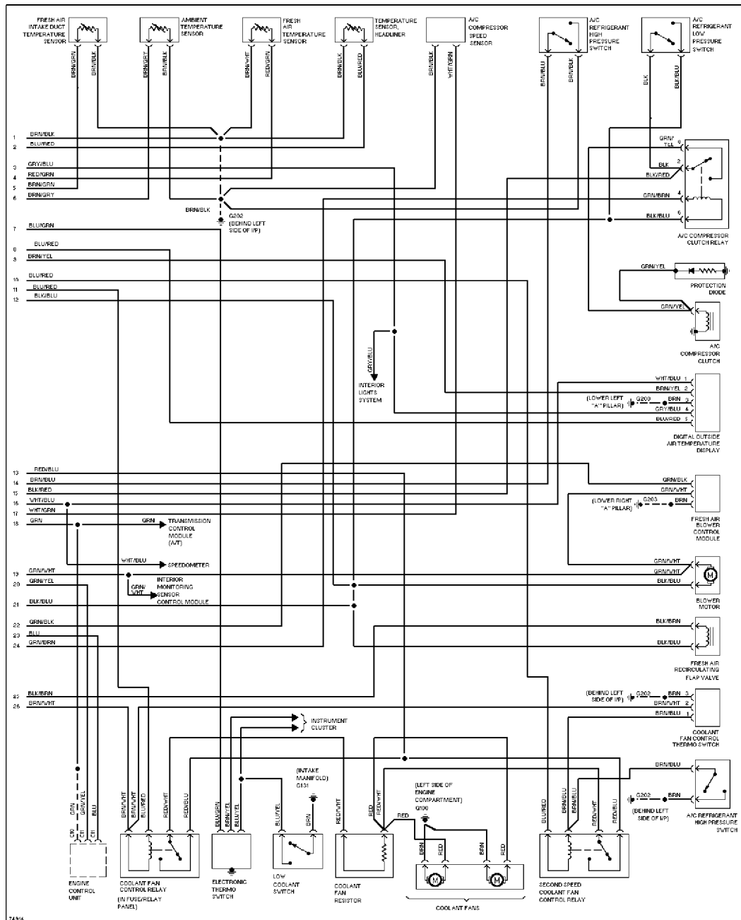
Fig. 9: Automatic A/C-Heater System Wiring Diagram (1995 (Late Production) & 1996 - 2 Of 2)
