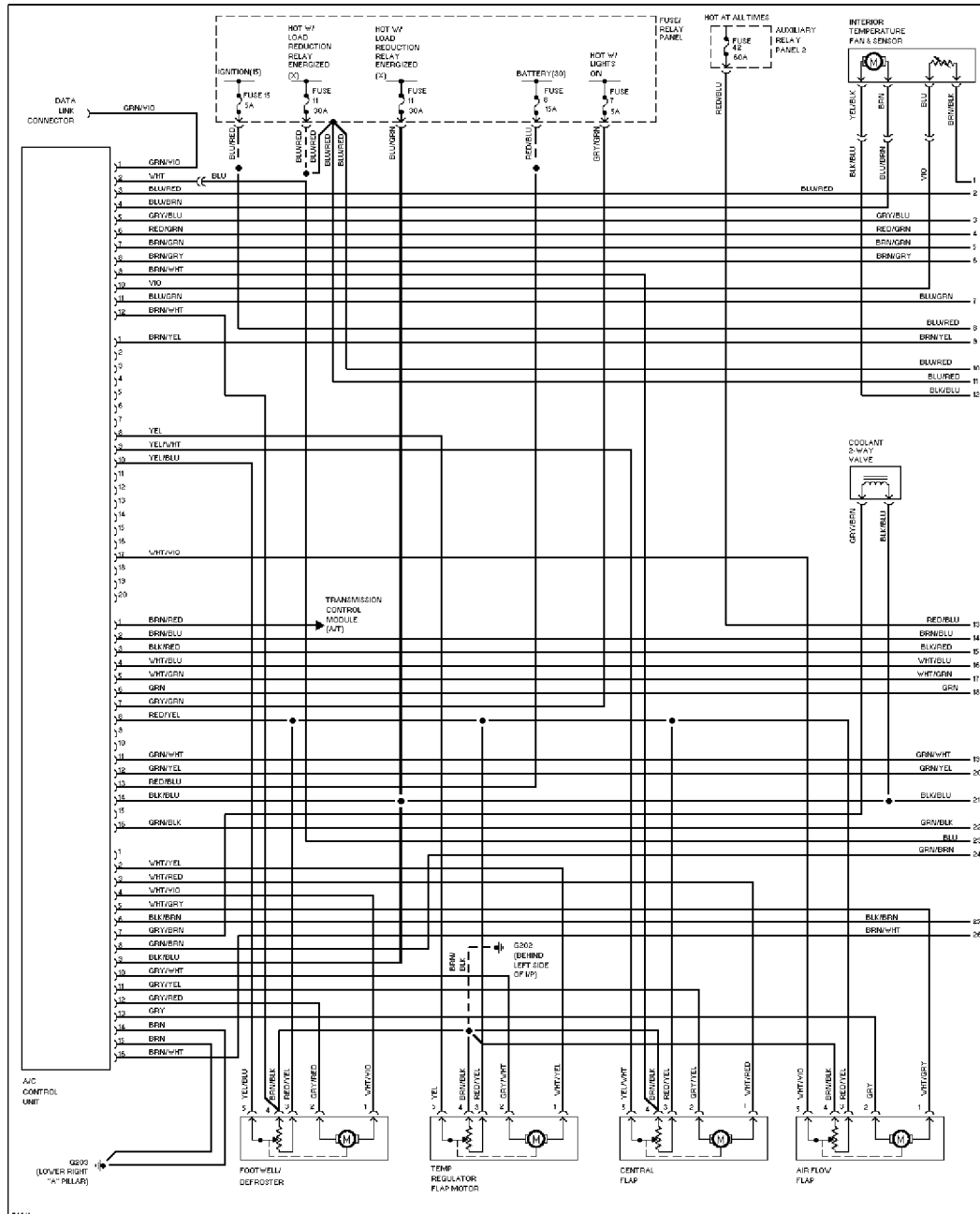
Fig. 6: Automatic A/C-Heater System Wiring Diagram (1995 (Early Production) - 1 Of 2)
