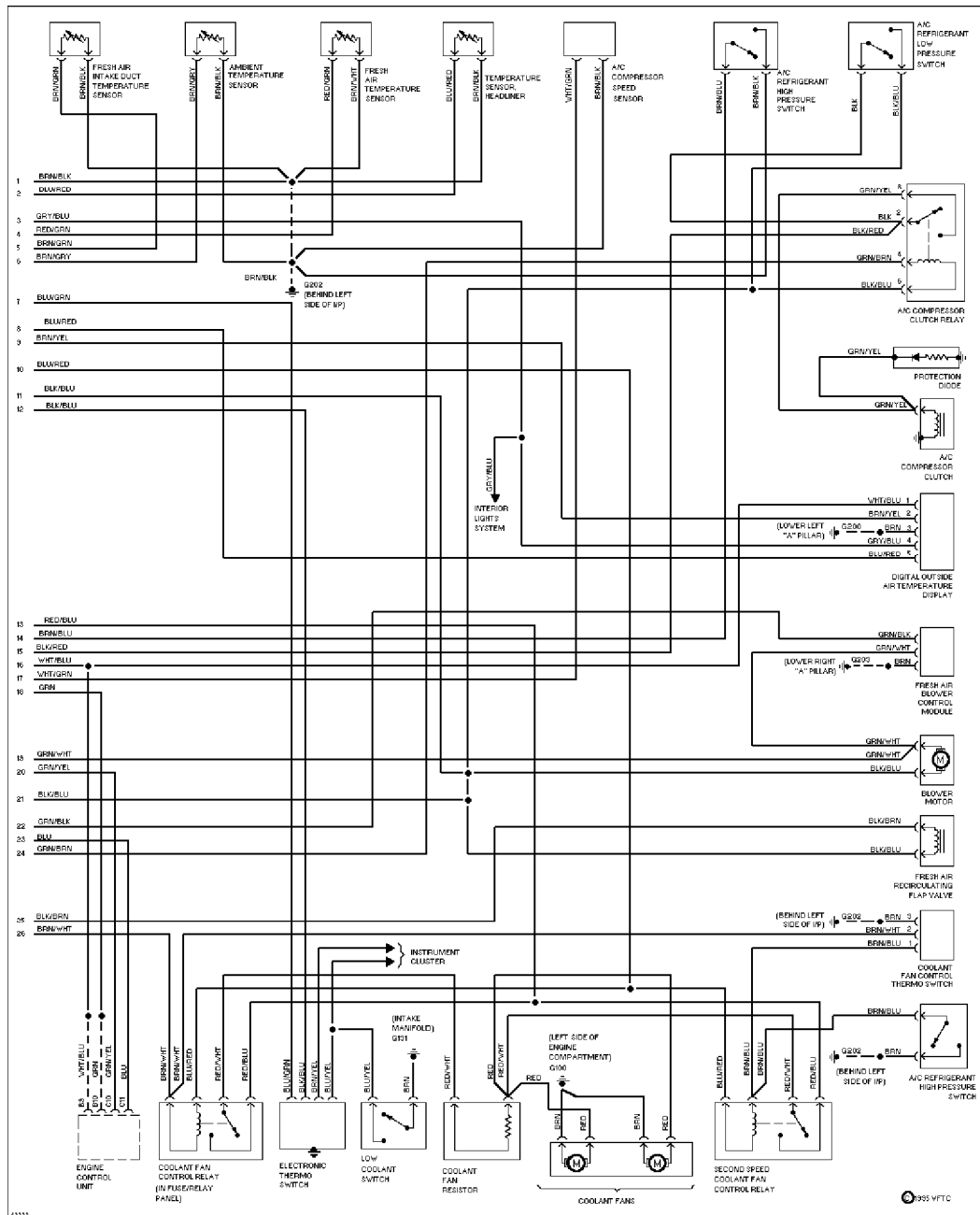
Fig. 7: A/C-Heater System Wiring Diagram (100 CS - 2 Of 2)
